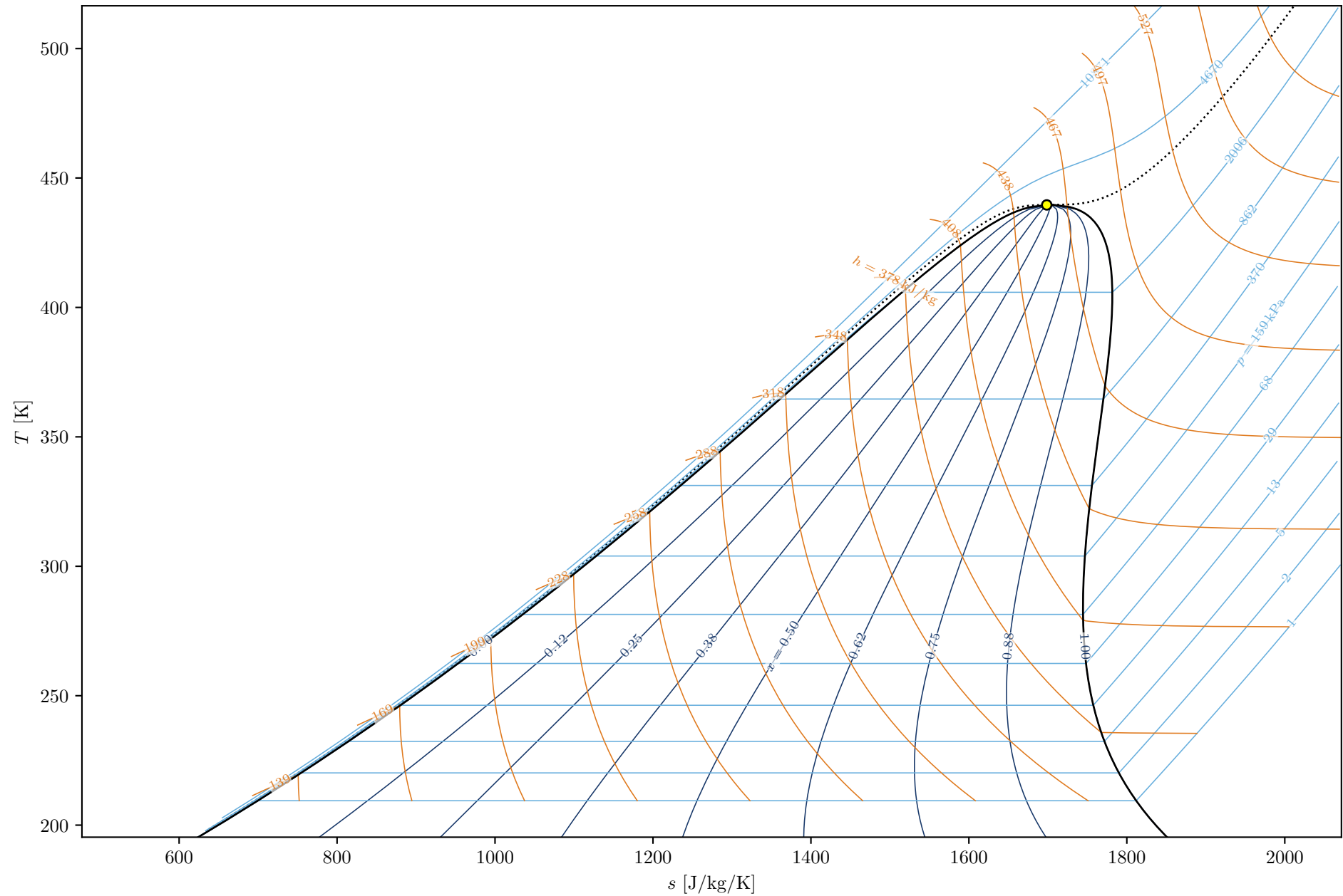
Thermodynamic Diagram (TS) — R1233zd(E)
